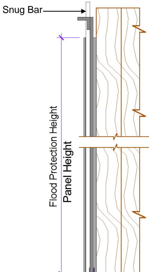
Section View
